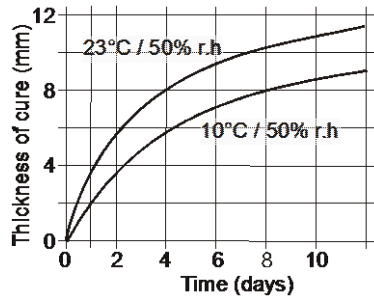
Diagram 1: Curing speed for Sikaflex®-221
